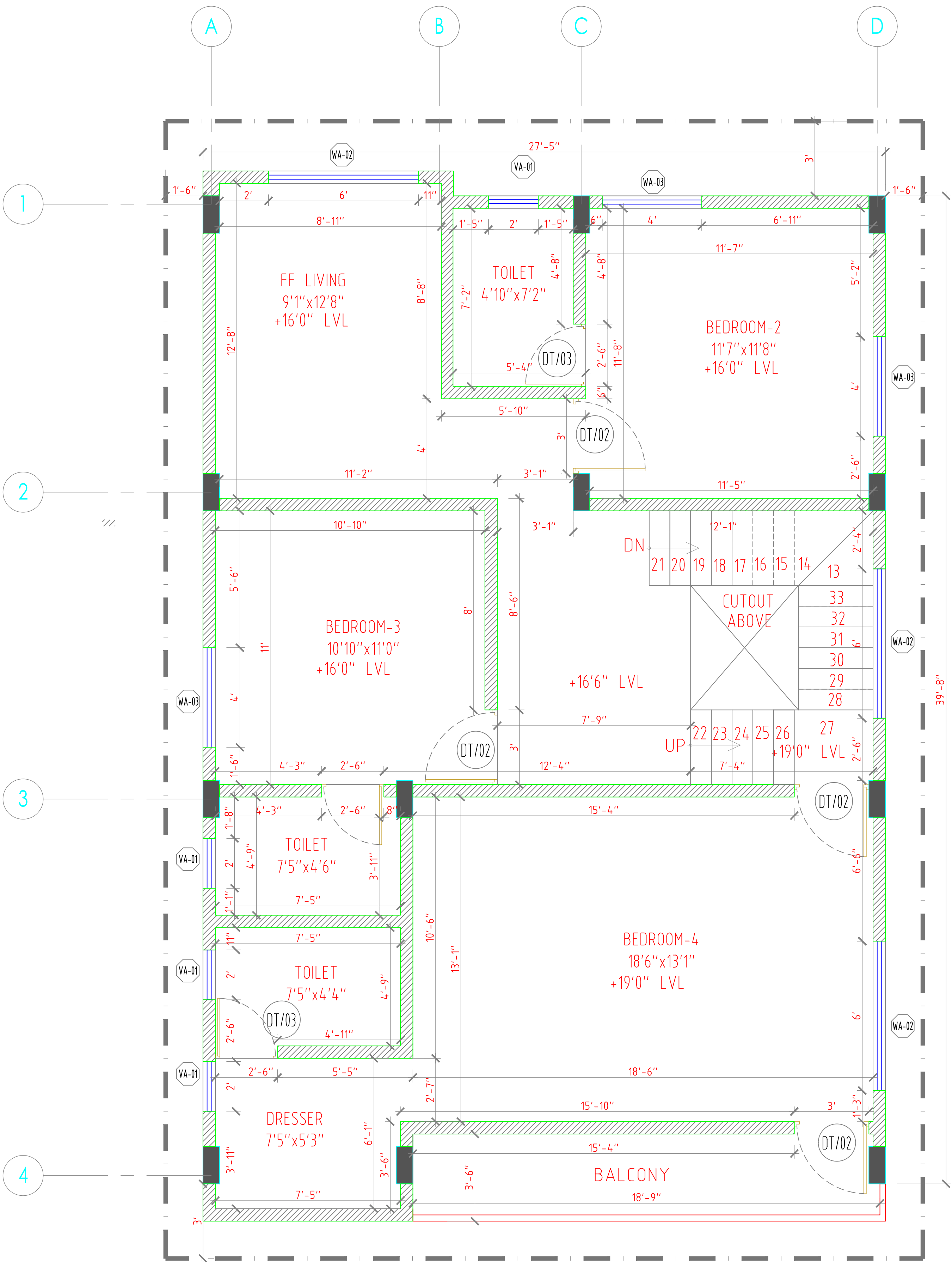
FIRST FLOOR PLAN 01
